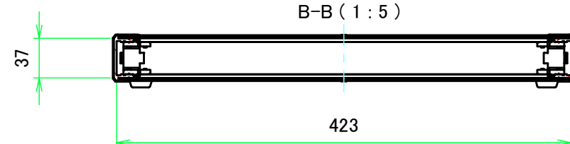
B-B (1:5)
